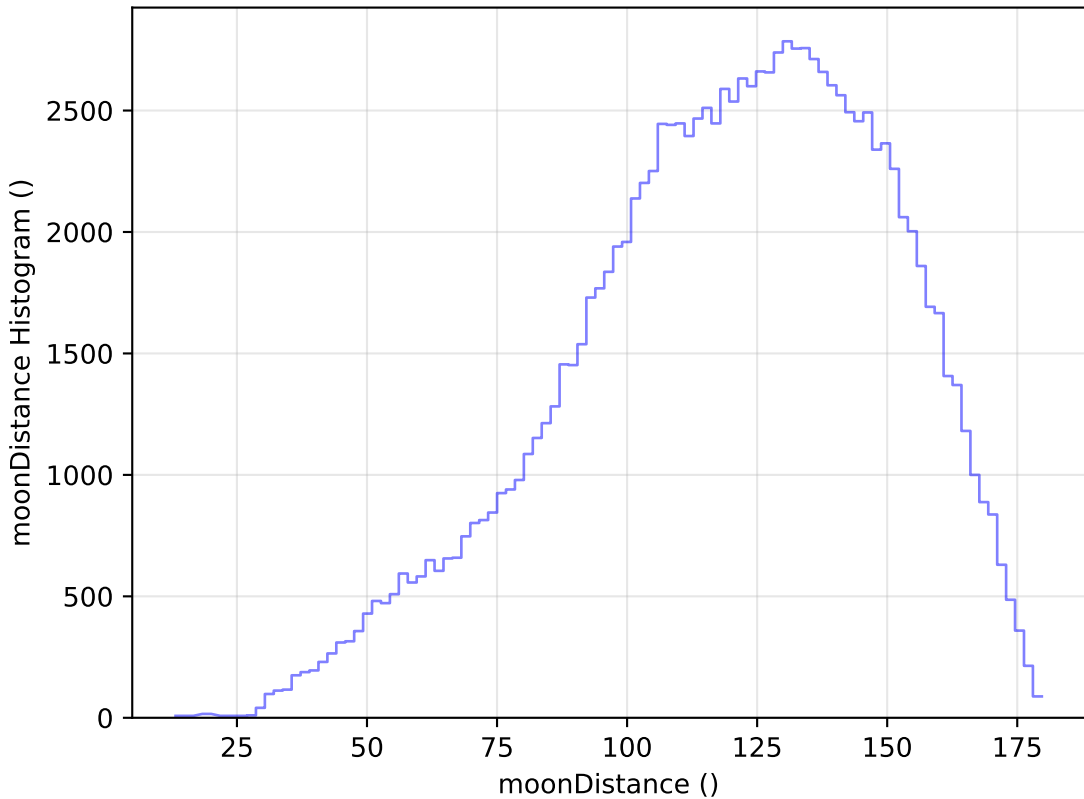
roll_pause_mjdp365_v3.4_10yrs WFD u band: moonDistance Histogram
