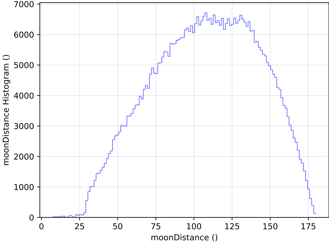
roll_pause_mjdp365_v3.4_10yrs WFD r band: moonDistance Histogram
