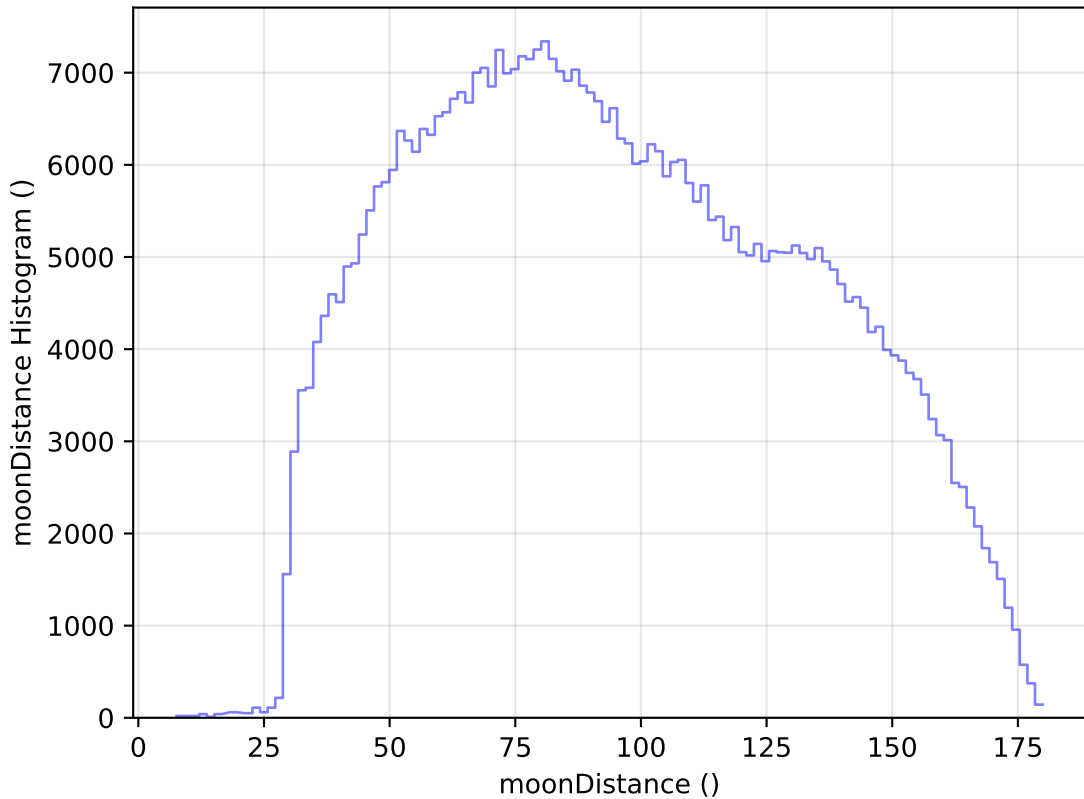
roll_pause_mjdp365_v3.4_10yrs WFD i band: moonDistance Histogram
