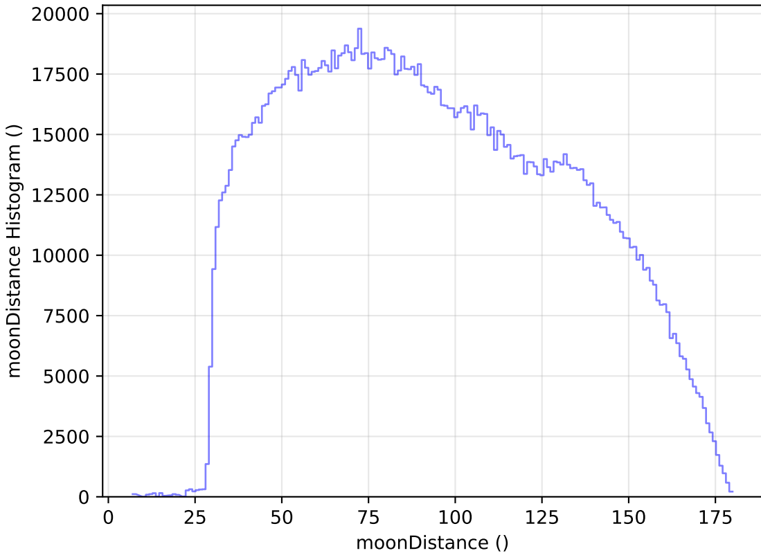
roll_pause_mjdp365_v3.4_10yrs WFD all bands: moonDistance Histogram
