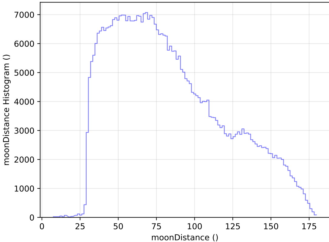
roll_pause_mjdp365_v3.4_10yrs All sky z band: moonDistance Histogram
