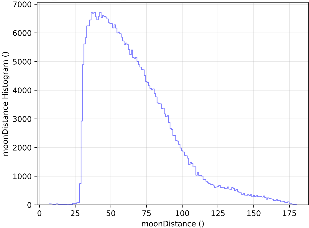
roll_pause_mjdp365_v3.4_10yrs All sky y band: moonDistance Histogram
