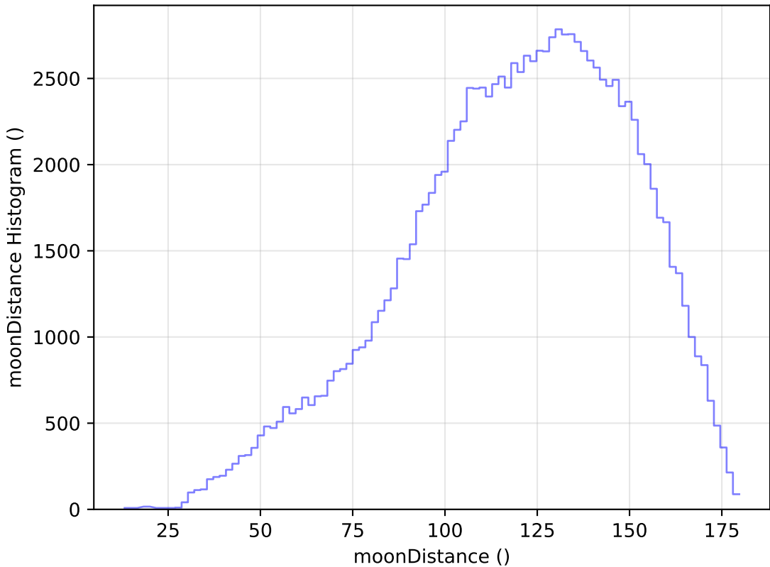
roll_pause_mjdp365_v3.4_10yrs All sky u band: moonDistance Histogram
