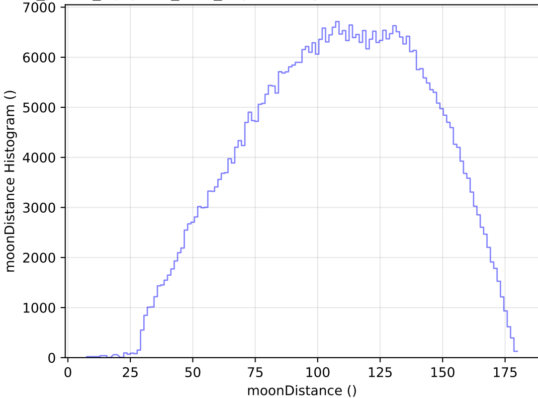
roll_pause_mjdp365_v3.4_10yrs All sky r band: moonDistance Histogram
