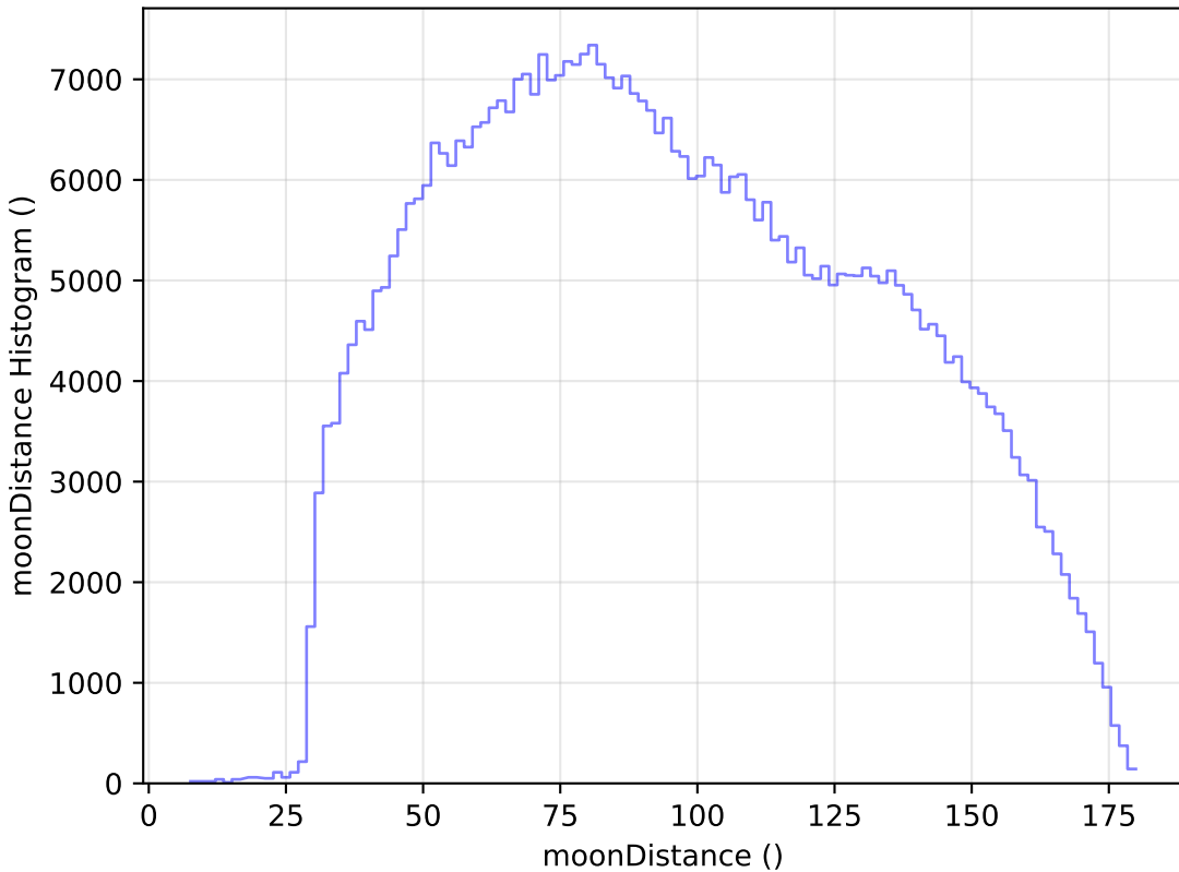
roll_pause_mjdp365_v3.4_10yrs All sky i band: moonDistance Histogram
