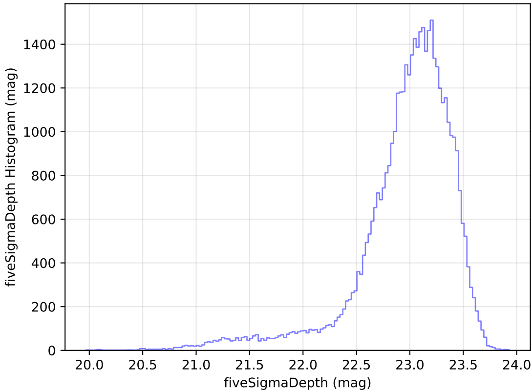
roll_pause_mjdp365_v3.4_10yrs Yr 1 z band: fiveSigmaDepth Histogram
