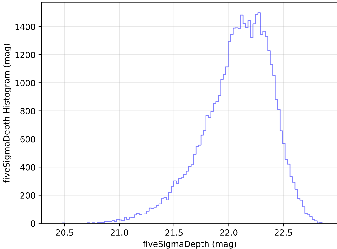
roll_pause_mjdp365_v3.4_10yrs Yr 1 y band: fiveSigmaDepth Histogram
