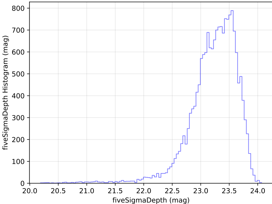
roll_pause_mjdp365_v3.4_10yrs Yr 1 u band: fiveSigmaDepth Histogram
