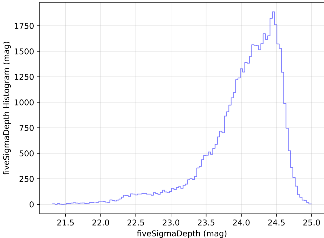
roll_pause_mjdp365_v3.4_10yrs Yr 1 r band: fiveSigmaDepth Histogram
