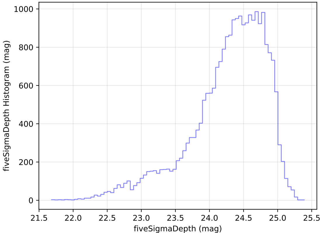
roll_pause_mjdp365_v3.4_10yrs Yr 1 g band: fiveSigmaDepth Histogram
