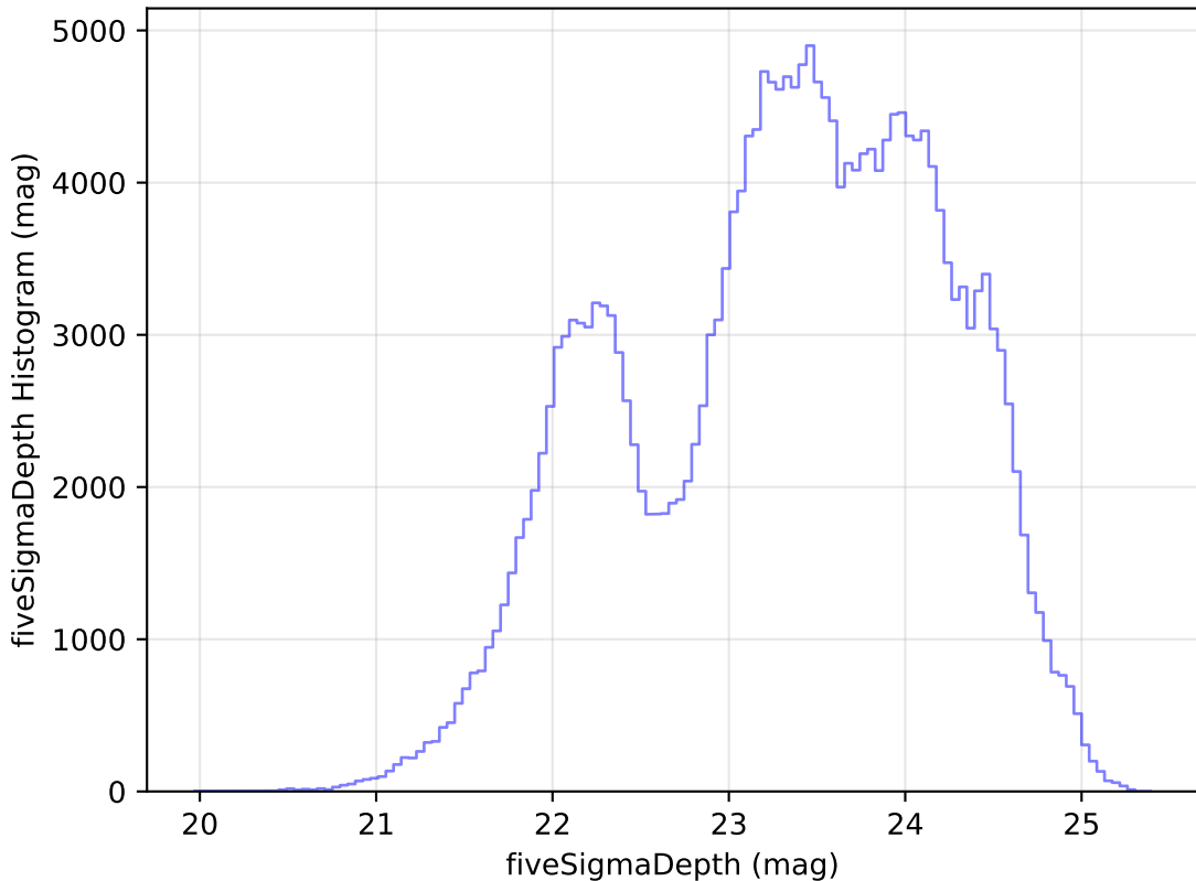
roll_pause_mjdp365_v3.4_10yrs Yr 1 all bands: fiveSigmaDepth Histogram
