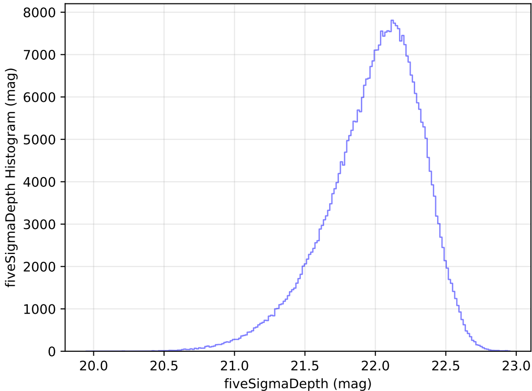
roll_pause_mjdp365_v3.4_10yrs WFD y band: fiveSigmaDepth Histogram
