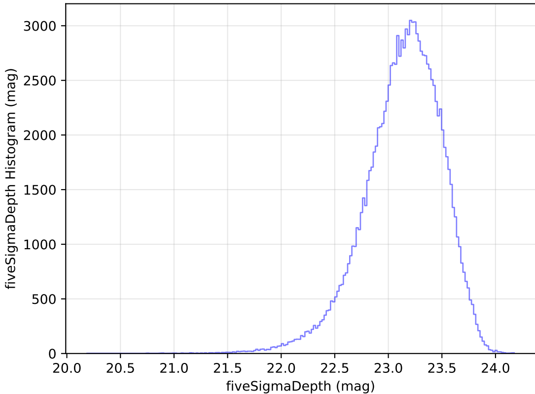
roll_pause_mjdp365_v3.4_10yrs WFD u band: fiveSigmaDepth Histogram
