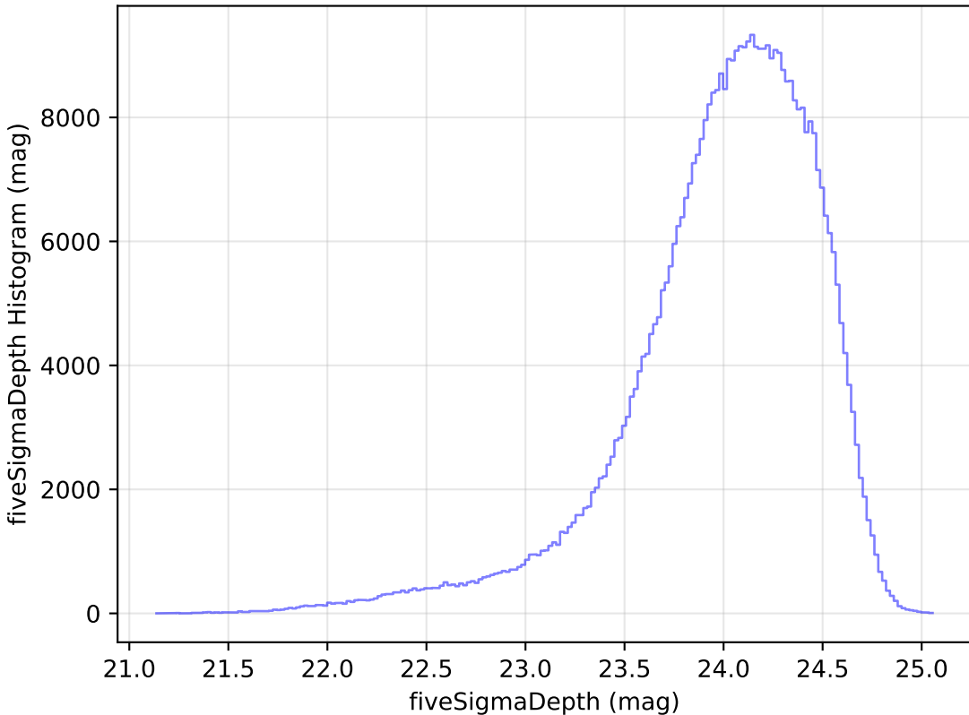
roll_pause_mjdp365_v3.4_10yrs WFD r band: fiveSigmaDepth Histogram
