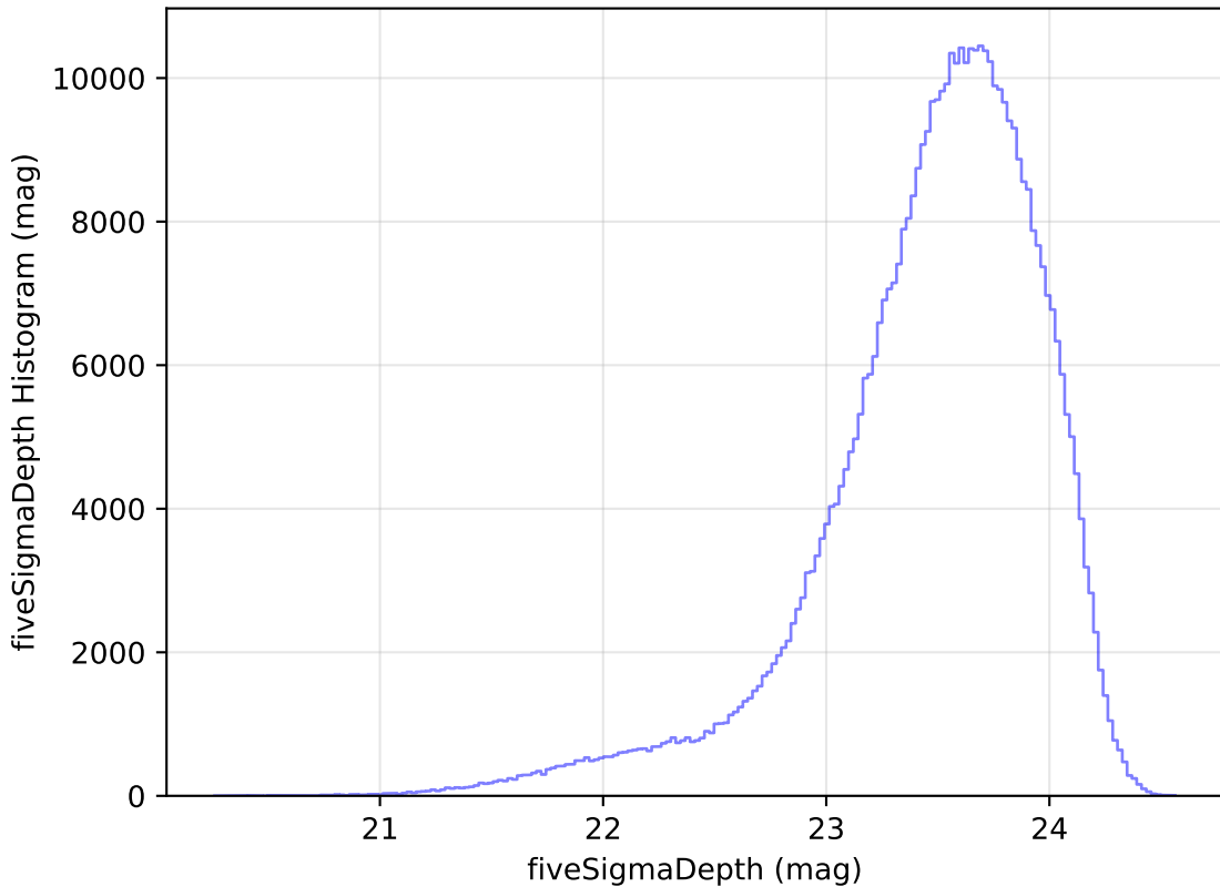
roll_pause_mjdp365_v3.4_10yrs WFD i band: fiveSigmaDepth Histogram
