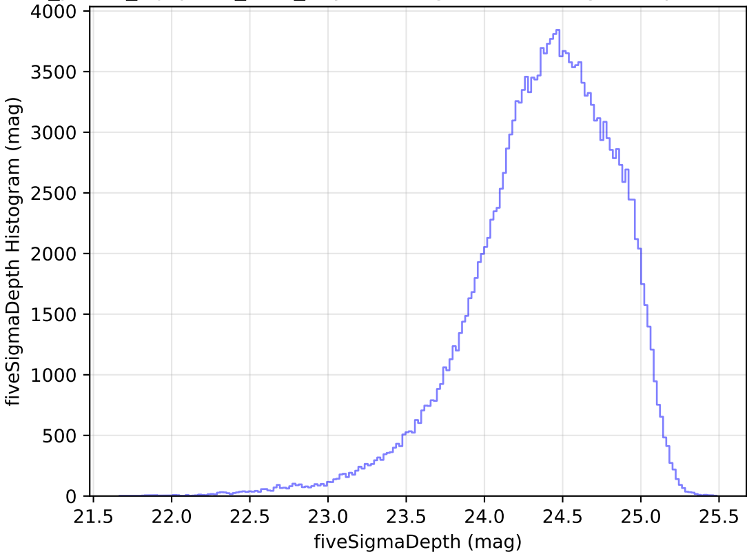
roll_pause_mjdp365_v3.4_10yrs WFD g band: fiveSigmaDepth Histogram
