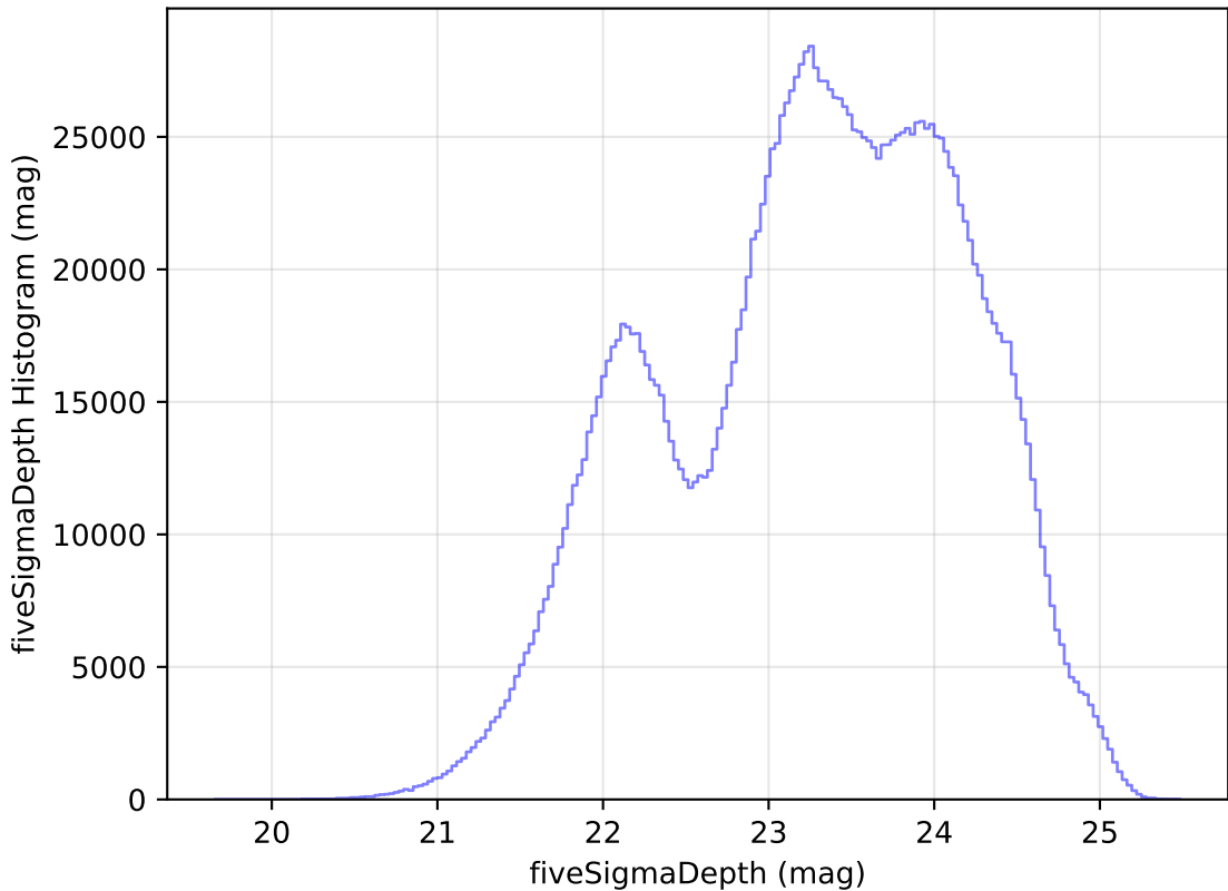
roll_pause_mjdp365_v3.4_10yrs WFD all bands: fiveSigmaDepth Histogram
