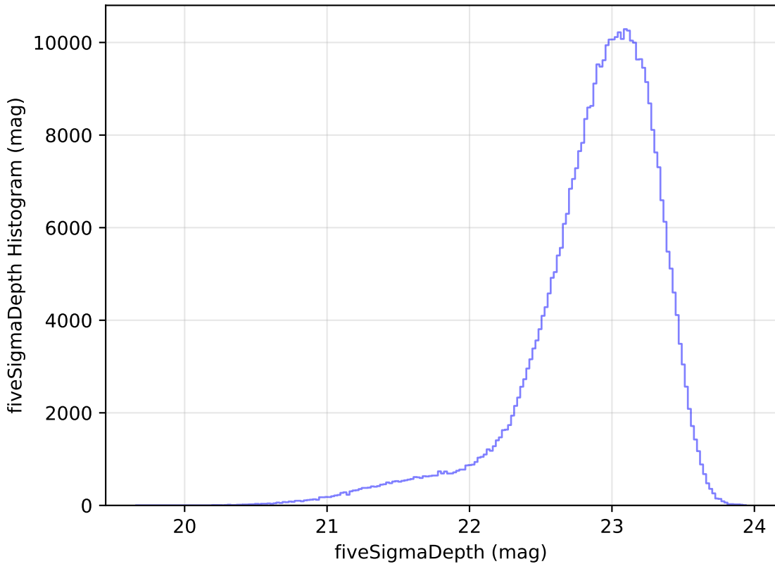
roll_pause_mjdp365_v3.4_10yrs All sky z band: fiveSigmaDepth Histogram
