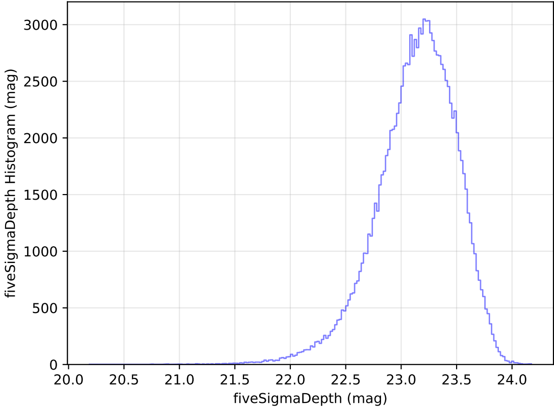
roll_pause_mjdp365_v3.4_10yrs All sky u band: fiveSigmaDepth Histogram
