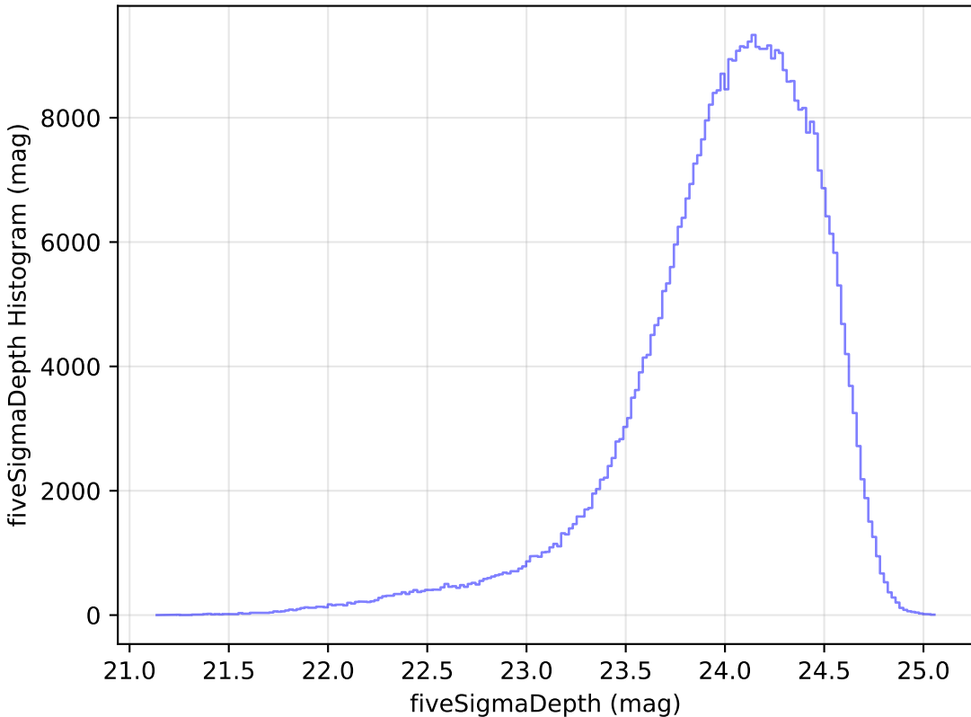
roll_pause_mjdp365_v3.4_10yrs All sky r band: fiveSigmaDepth Histogram
