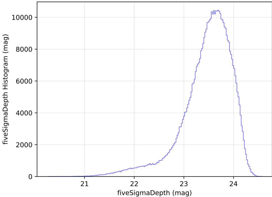
roll_pause_mjdp365_v3.4_10yrs All sky i band: fiveSigmaDepth Histogram
