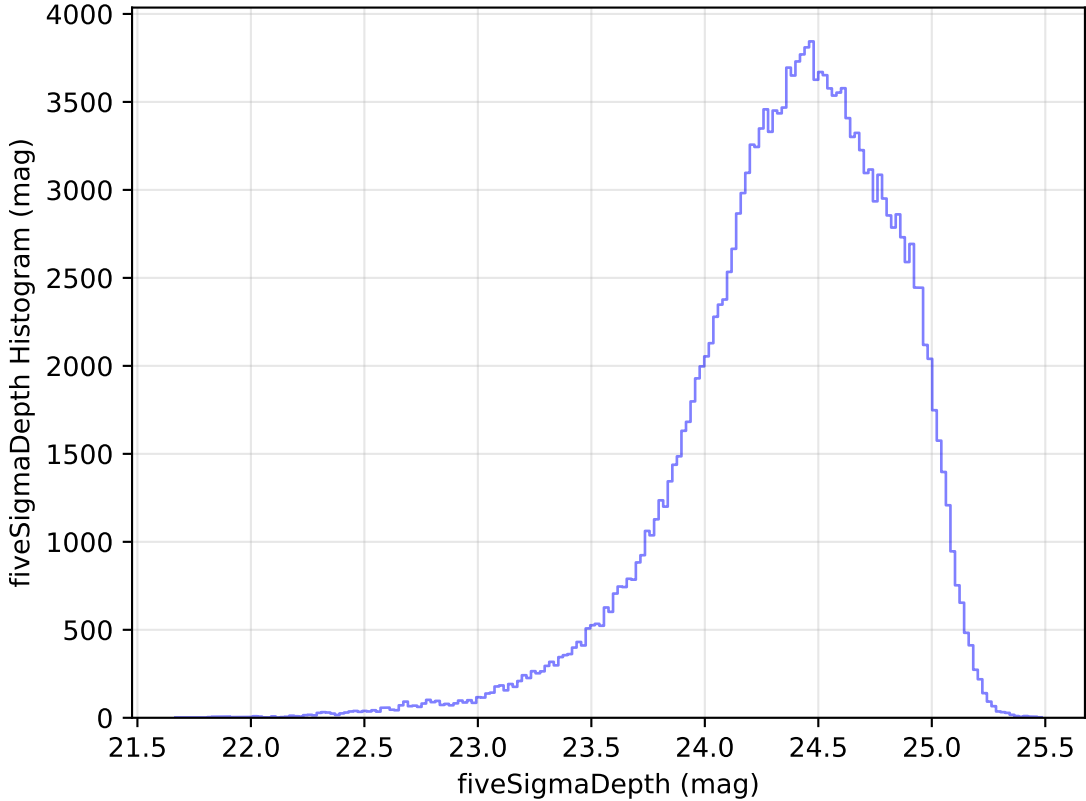
roll_pause_mjdp365_v3.4_10yrs All sky g band: fiveSigmaDepth Histogram
