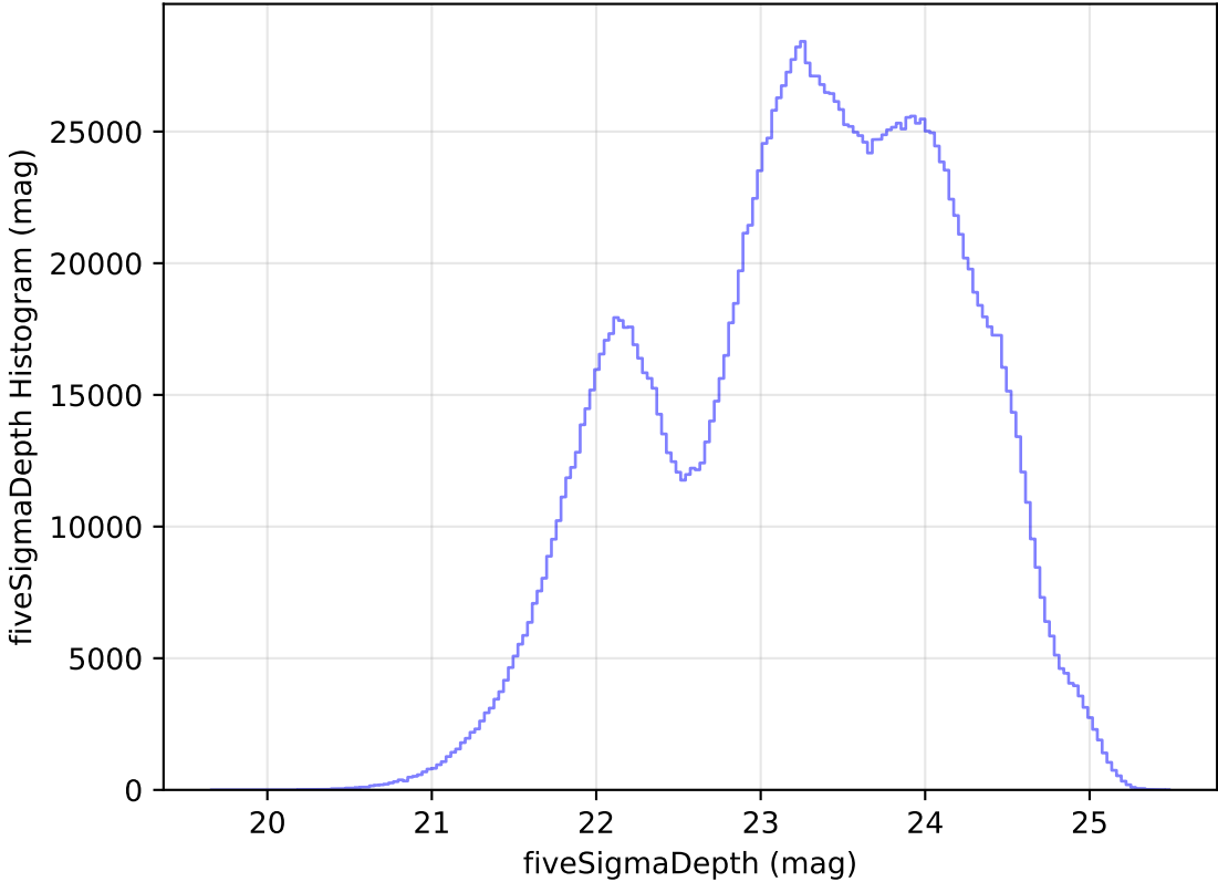
roll_pause_mjdp365_v3.4_10yrs All sky all bands: fiveSigmaDepth Histogram
