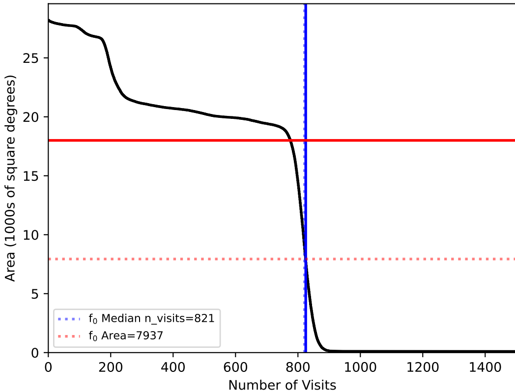
roll_pause_mjdp365_v3.4_10yrs All sky: fO
