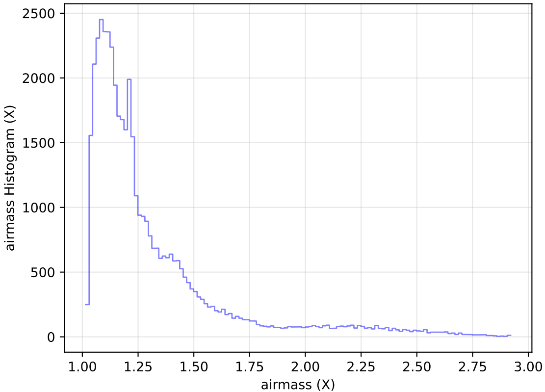
roll_pause_mjdp365_v3.4_10yrs Yr 1 z band: airmass Histogram
