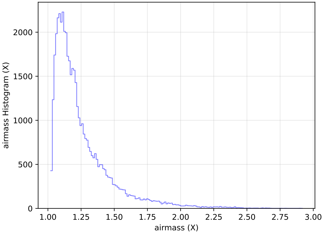
roll_pause_mjdp365_v3.4_10yrs Yr 1 y band: airmass Histogram
