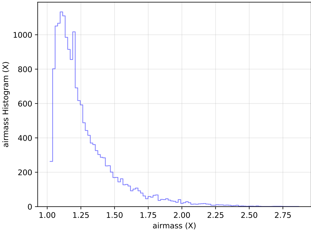
roll_pause_mjdp365_v3.4_10yrs Yr 1 u band: airmass Histogram
