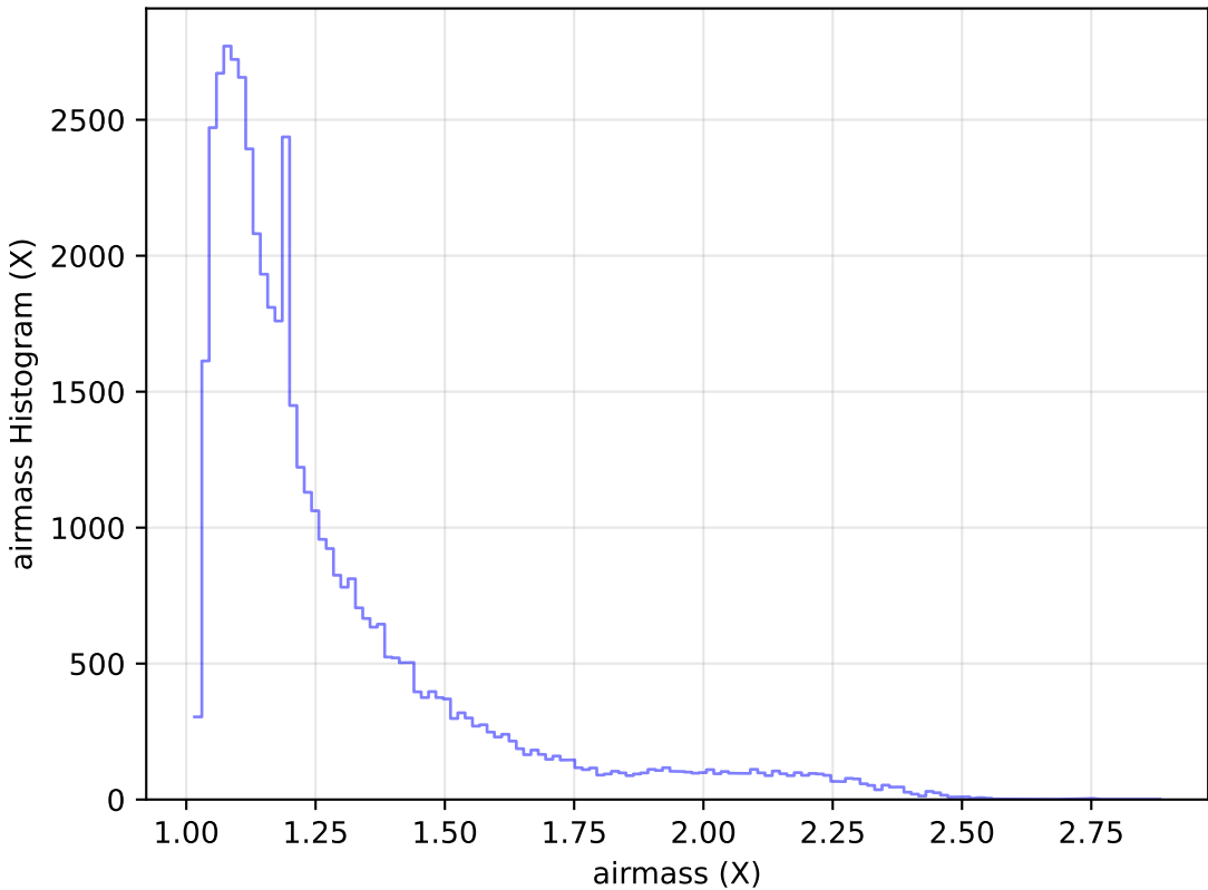
roll_pause_mjdp365_v3.4_10yrs Yr 1 r band: airmass Histogram
