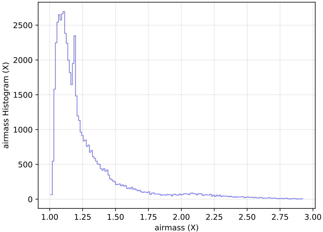
roll_pause_mjdp365_v3.4_10yrs Yr 1 i band: airmass Histogram
