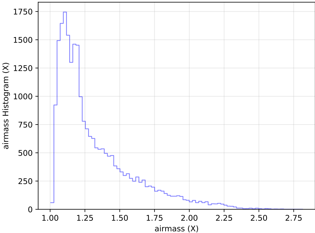
roll_pause_mjdp365_v3.4_10yrs Yr 1 g band: airmass Histogram
