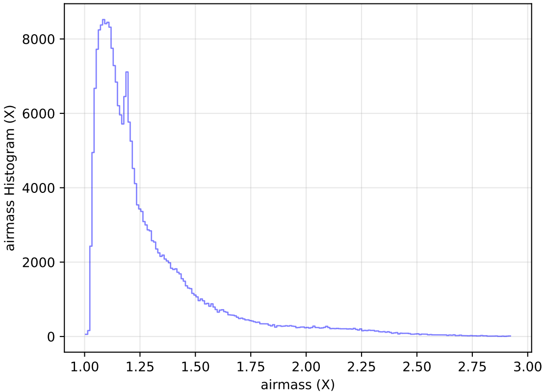
roll_pause_mjdp365_v3.4_10yrs Yr 1 all bands: airmass Histogram
