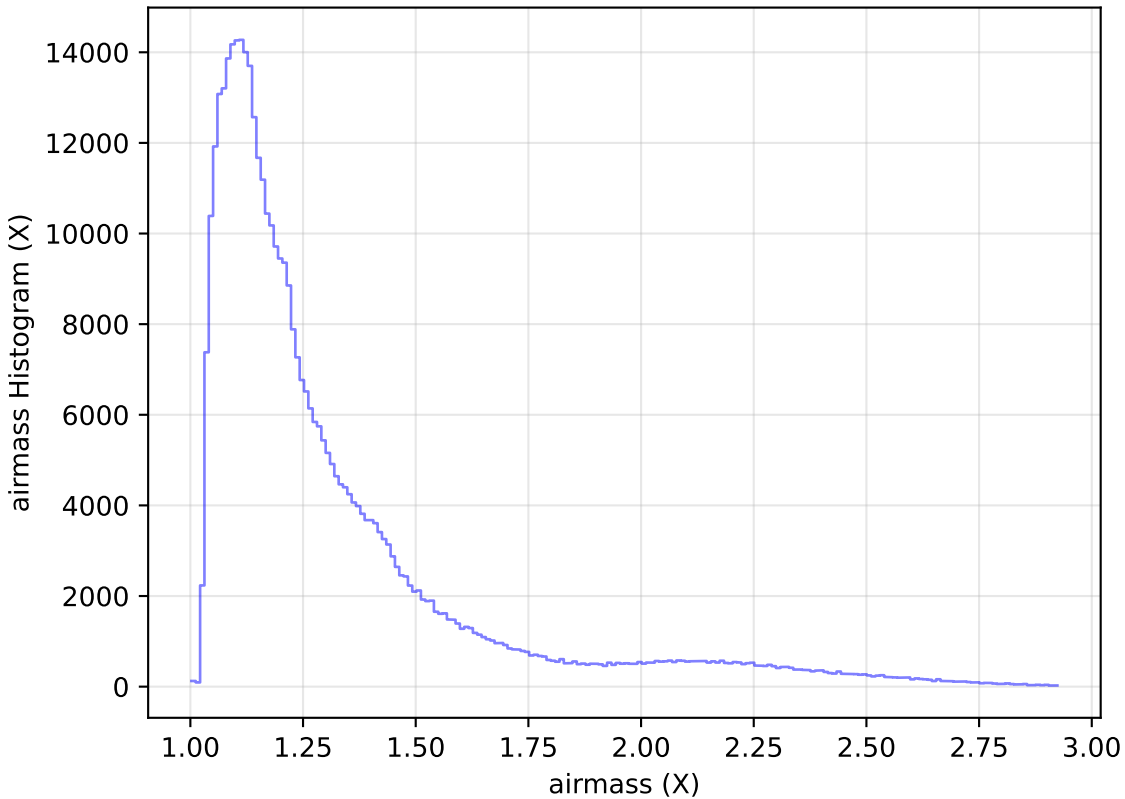
roll_pause_mjdp365_v3.4_10yrs WFD z band: airmass Histogram
