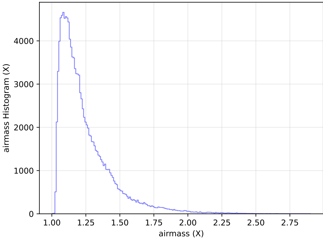
roll_pause_mjdp365_v3.4_10yrs WFD u band: airmass Histogram
