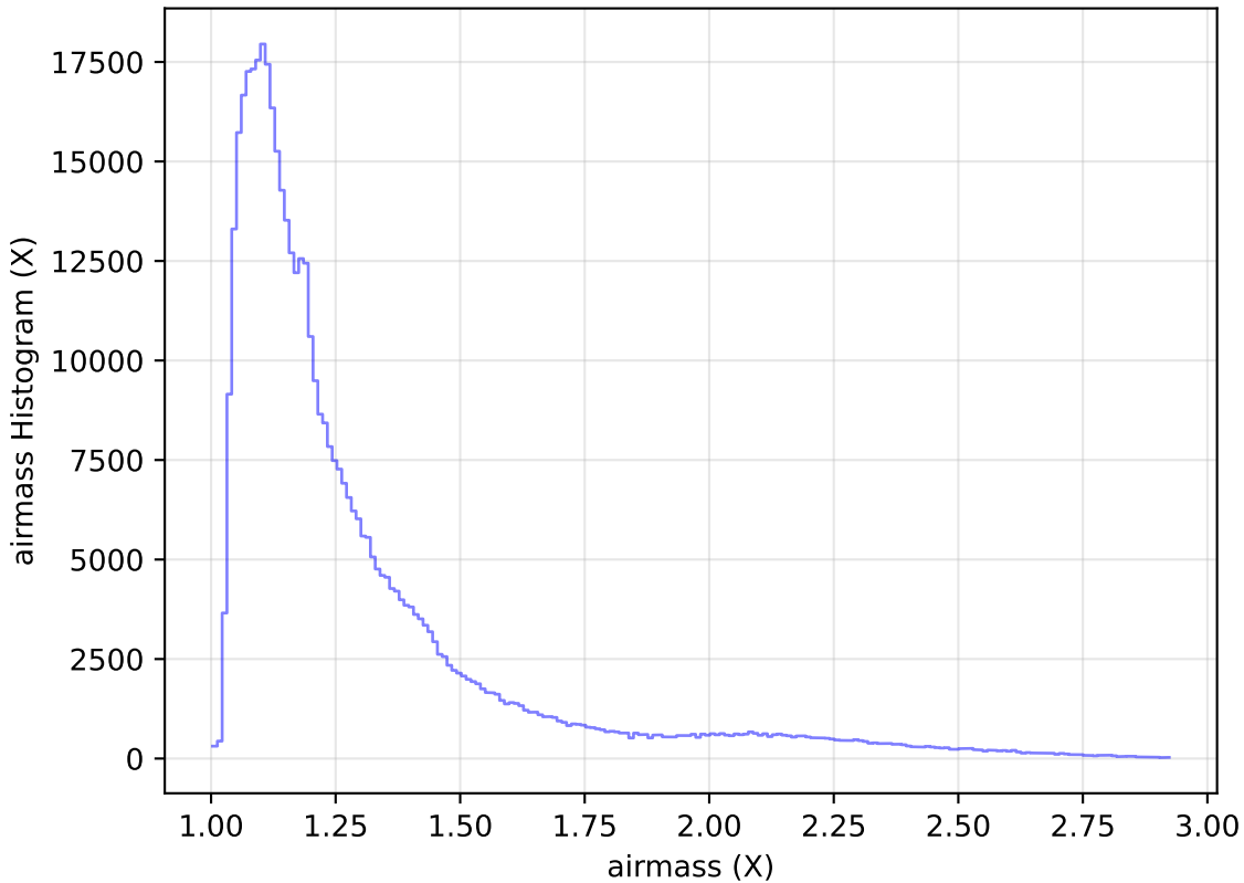
roll_pause_mjdp365_v3.4_10yrs WFD i band: airmass Histogram
