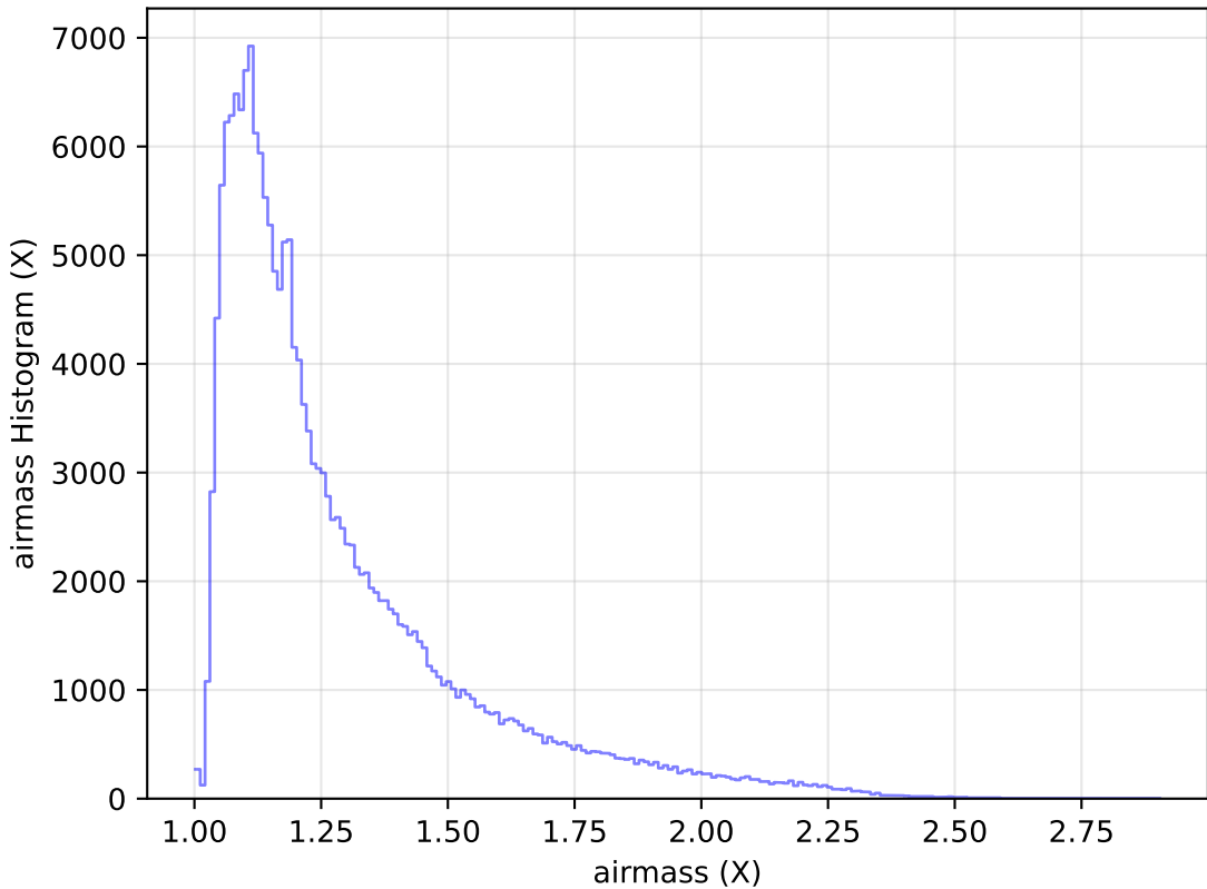
roll_pause_mjdp365_v3.4_10yrs WFD g band: airmass Histogram
