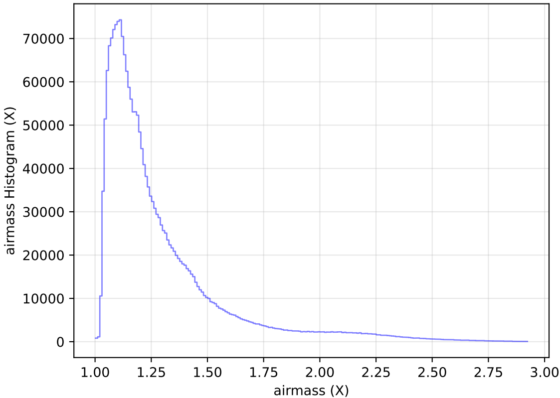
roll_pause_mjdp365_v3.4_10yrs WFD all bands: airmass Histogram
