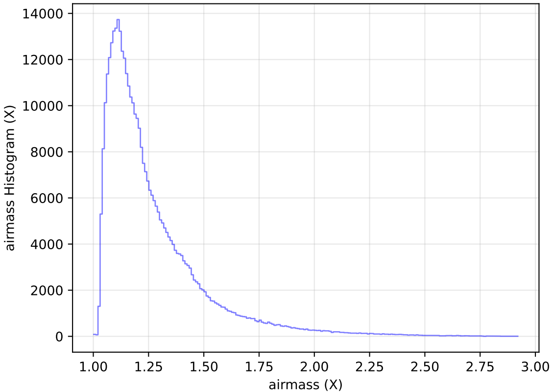
roll_pause_mjdp365_v3.4_10yrs All sky y band: airmass Histogram
