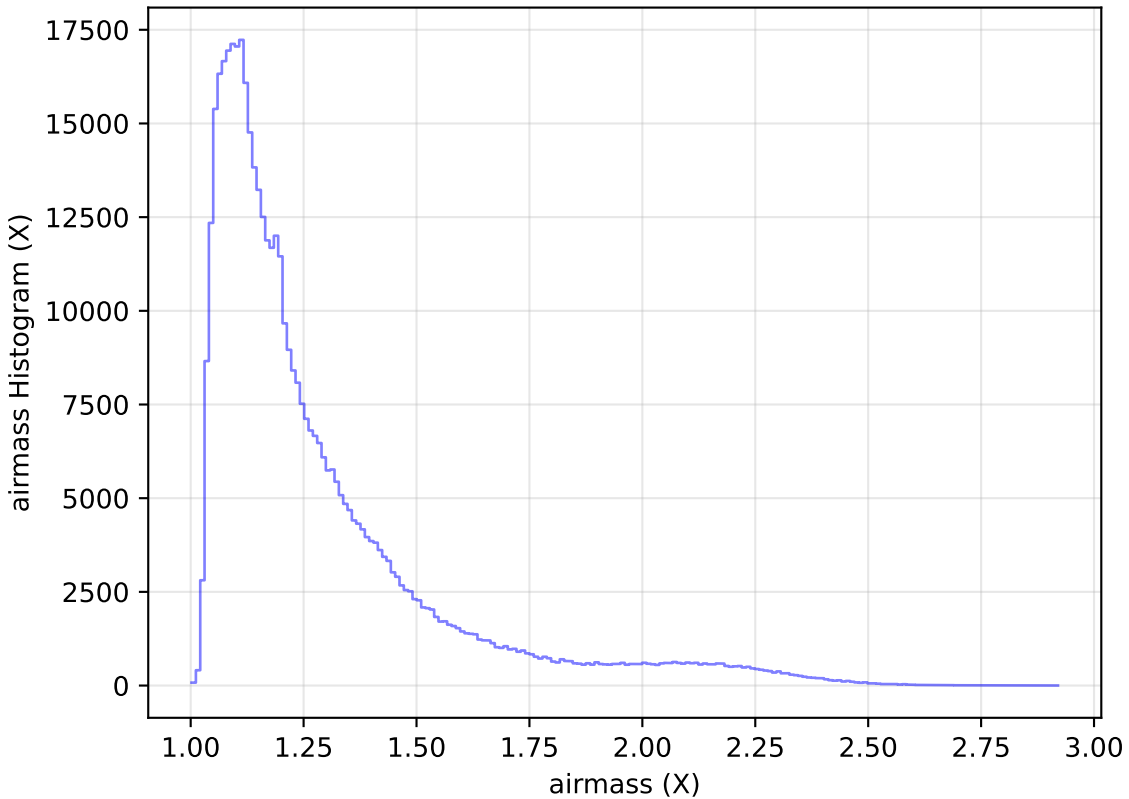
roll_pause_mjdp365_v3.4_10yrs All sky r band: airmass Histogram
