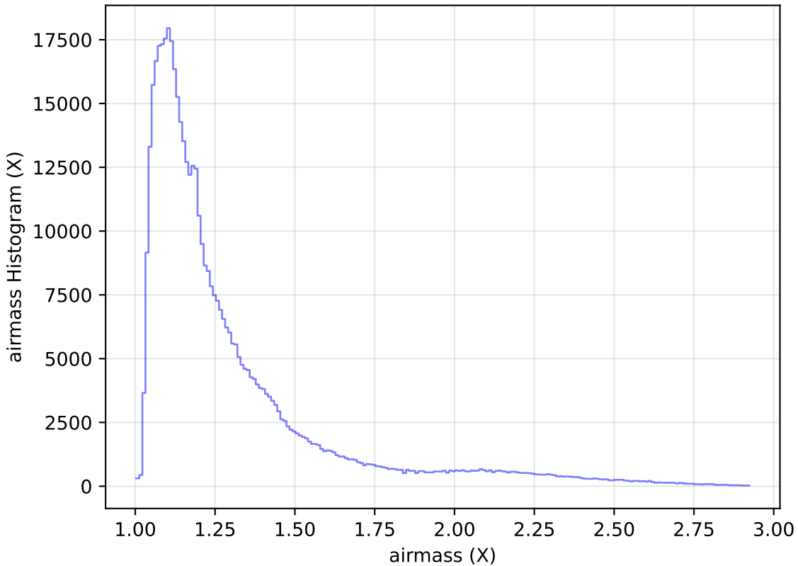
roll_pause_mjdp365_v3.4_10yrs All sky i band: airmass Histogram
