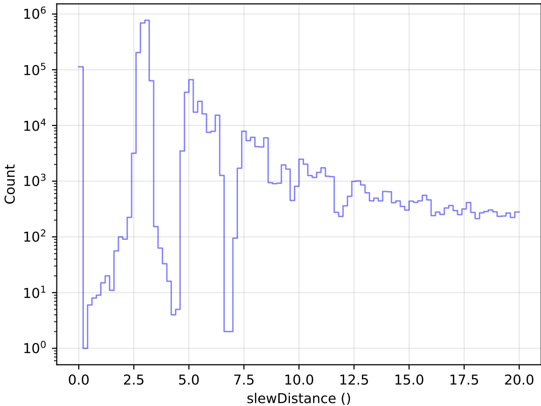
roll_pause_mjdp365_v3.4_10yrs All visits: Zoom Slew Distance Histogram
