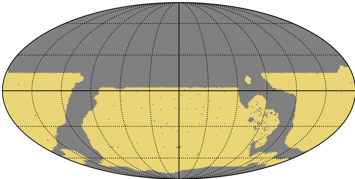
roll_pause_mjdp365_v3.4_10yrs WFD: RapidRevisits
