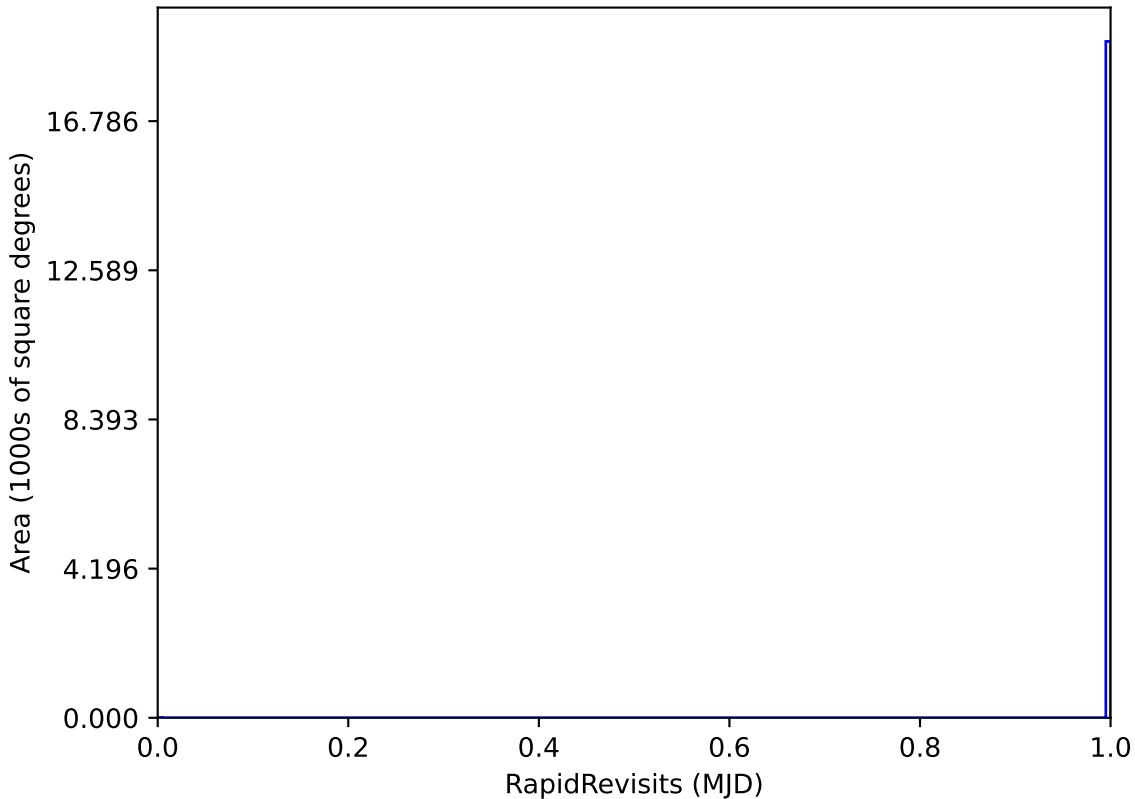
roll_pause_mjdp365_v3.4_10yrs WFD: RapidRevisits
