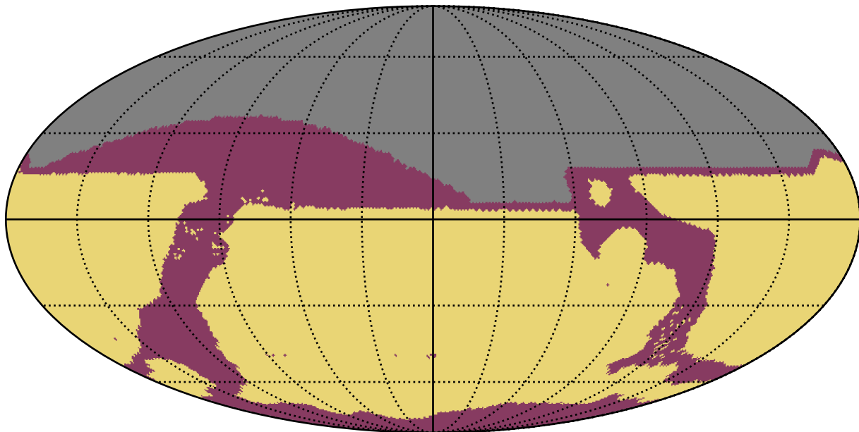
roll_pause_mjdp365_v3.4_10yrs All sky: RapidRevisits
