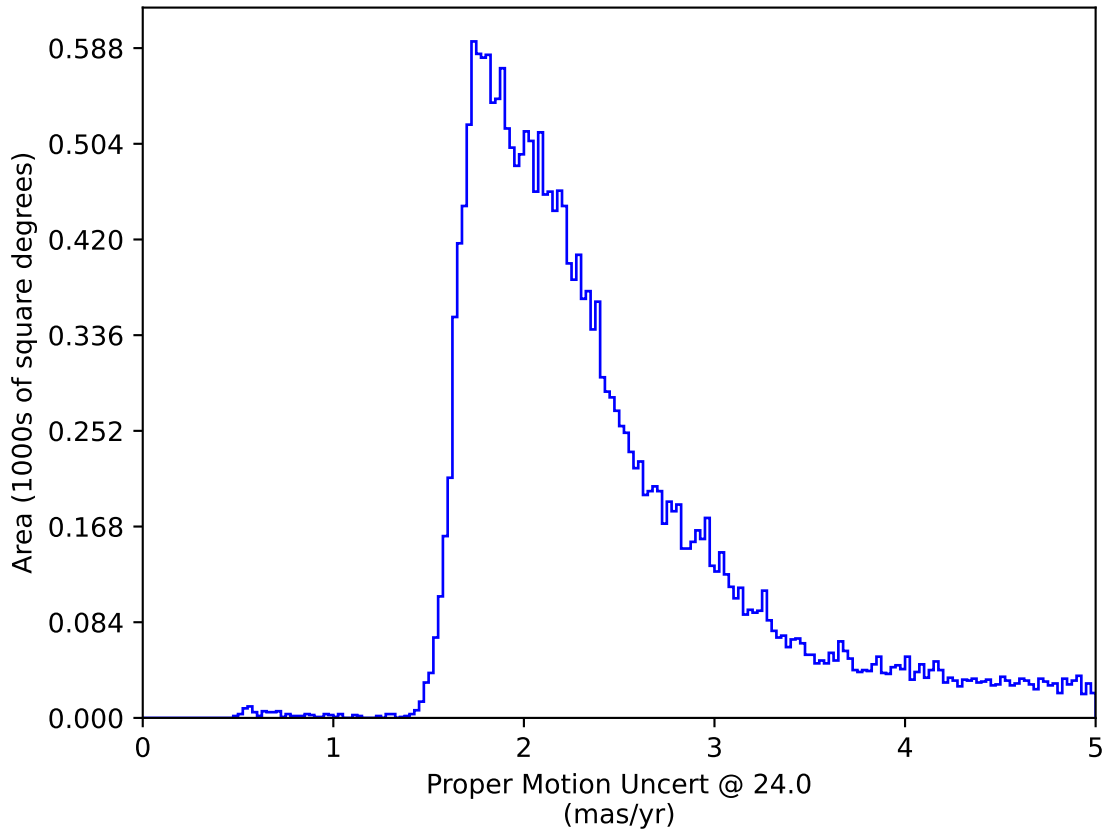
roll_pause_mjdp365_v3.4_10yrs All sky: Proper Motion Uncert @ 24.0
