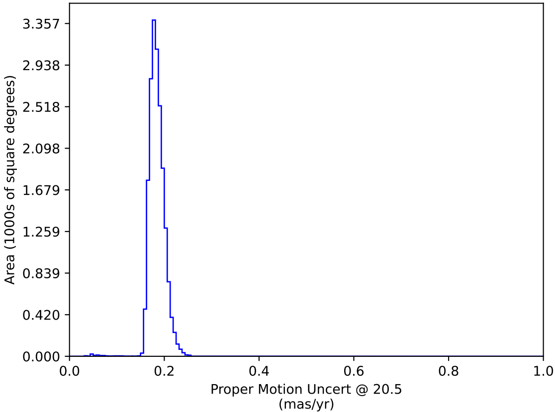
roll_pause_mjdp365_v3.4_10yrs WFD: Proper Motion Uncert @ 20.5
