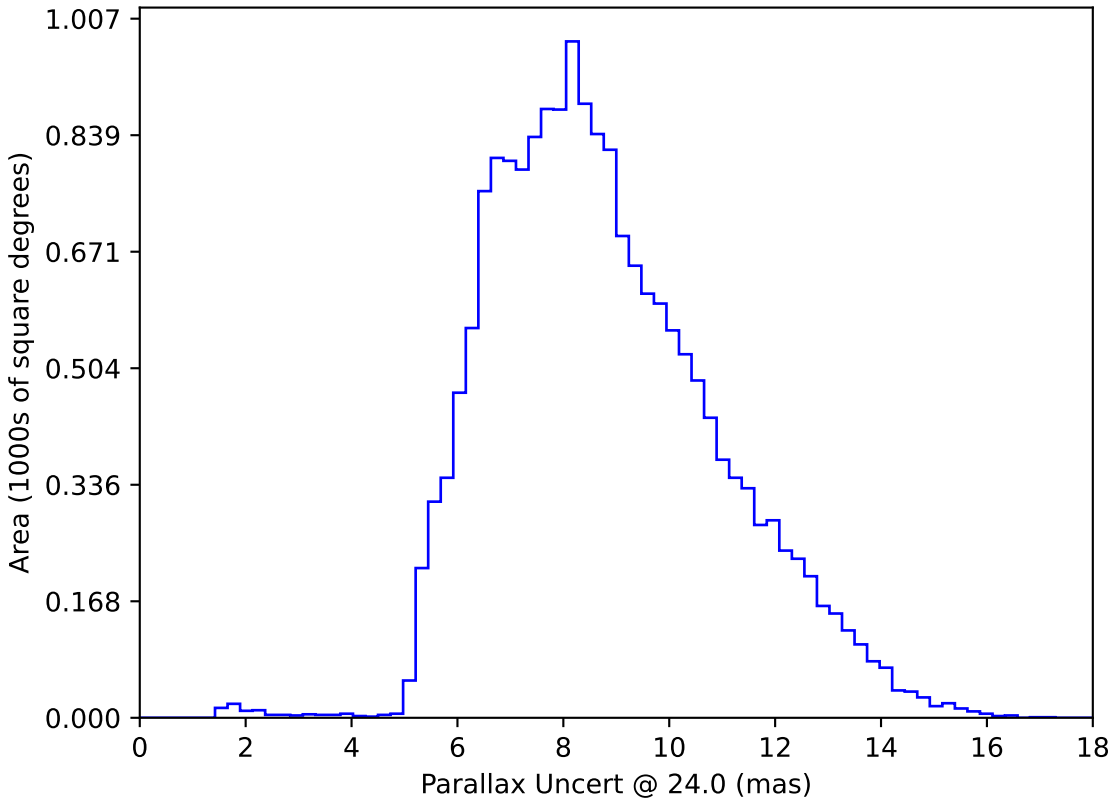
roll_pause_mjdp365_v3.4_10yrs WFD: Parallax Uncert @ 24.0
